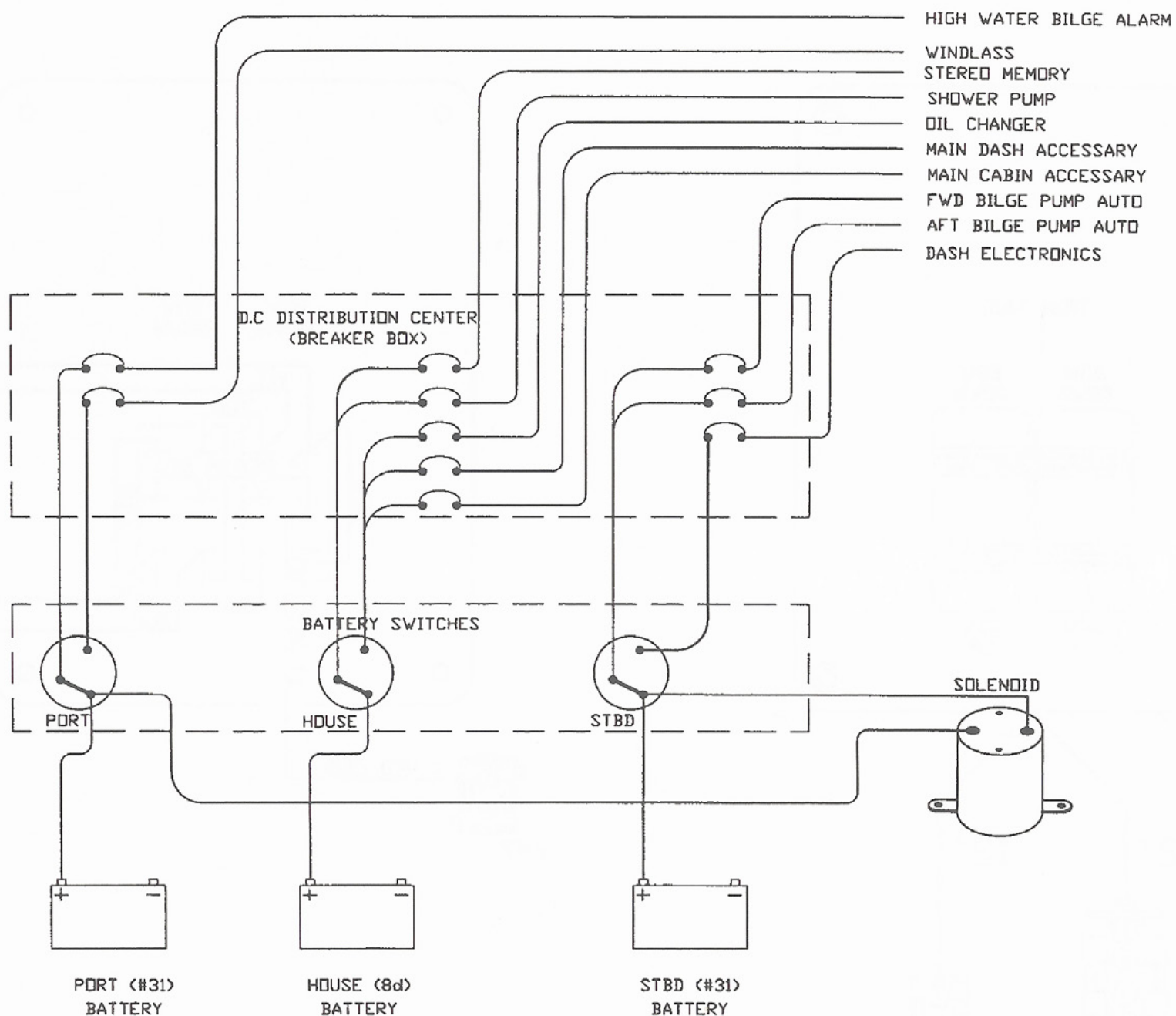
33 EXPRESS TYPICAL BATTERY MANAGEMENT PANEL CIRCUITRY
