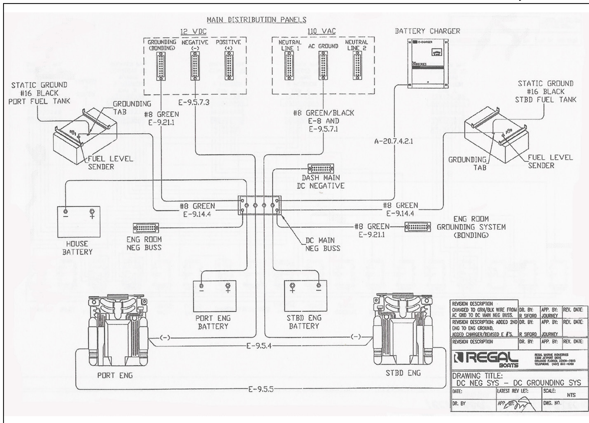
33 EXPRESS TYPICAL DC GROUND CIRCUITRY
